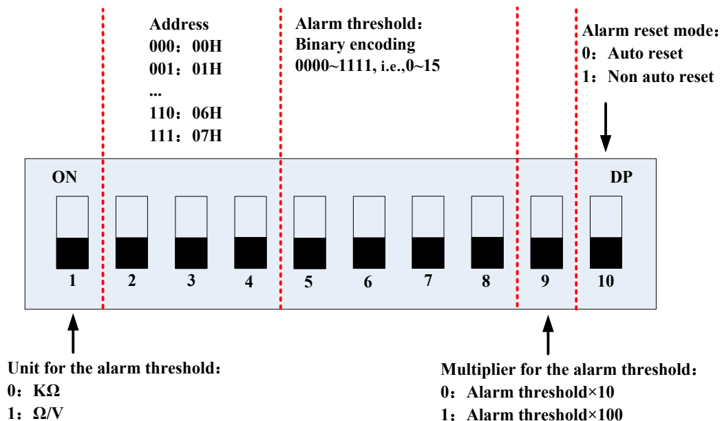
Figure 6: DIP Switch Parameter Configuration Diagram
