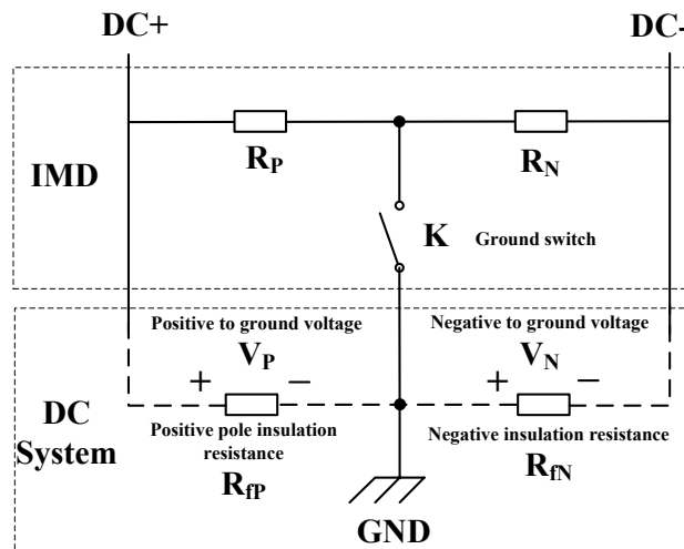
Figure 1: Schematic Diagram
